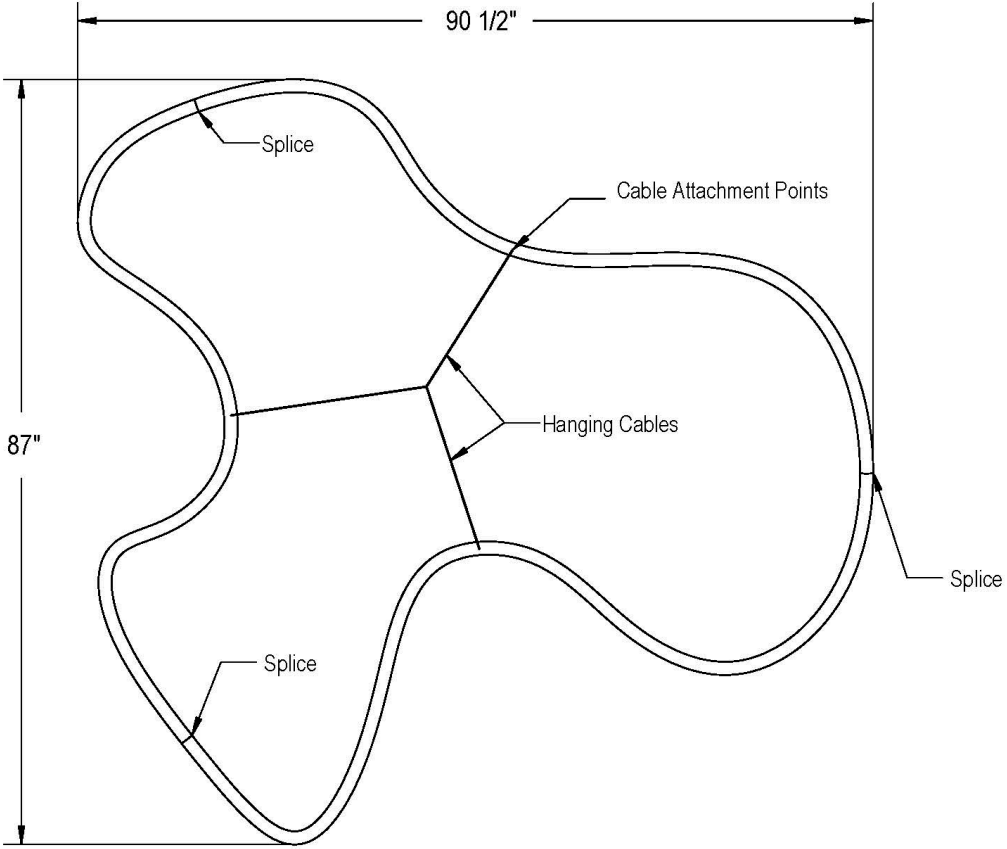
Top View Scale 1 : 16
