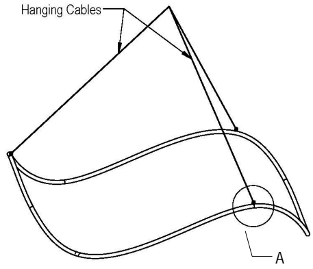
Isometric View Scale 1 : 32
