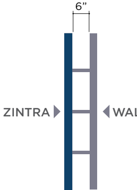
ZINTRA ACOUSTIC SOLUTIONS MOUNTED 6" AWAY FROM THE WALL NRC 0.95
