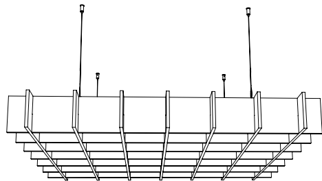
SQUARE 48" x 48" x 5.5" [1220mm x 1220mm x 140mm] Largest size possible 9' x 9' [2750mm x 2750mm]
