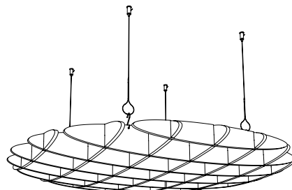
YOOFEO 48" DIA x 6.2" H [1220mm DIA x 157mm H] Largest size possible 9' x 9' [2750mm x 2750mm] DIA
