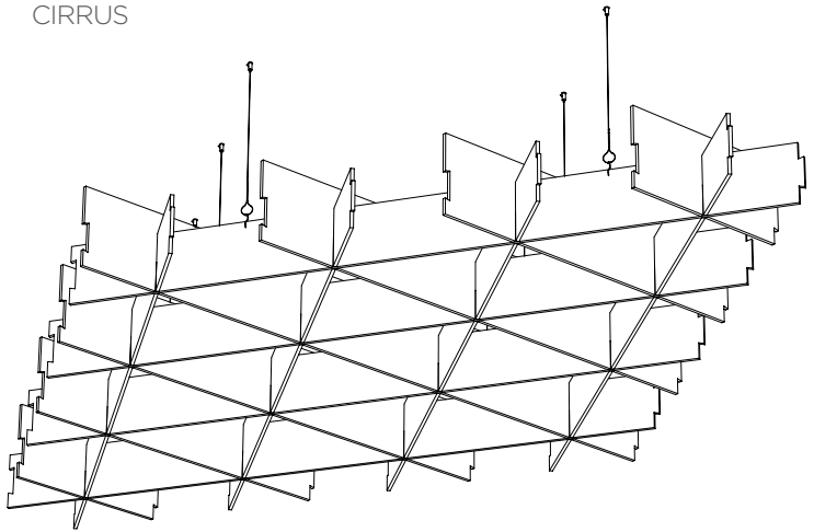
TYPICAL PERSPECTIVE FROM UNDERNEATH
