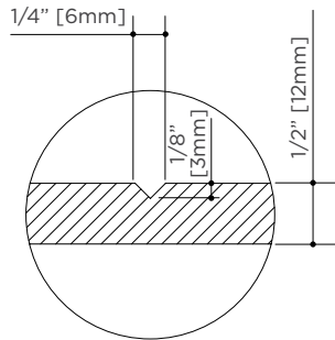
V-GROOVE DETAIL VIEW
