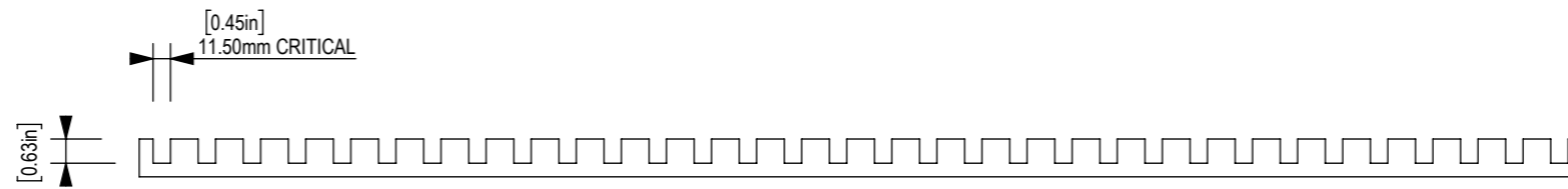
SIDE VIEW
